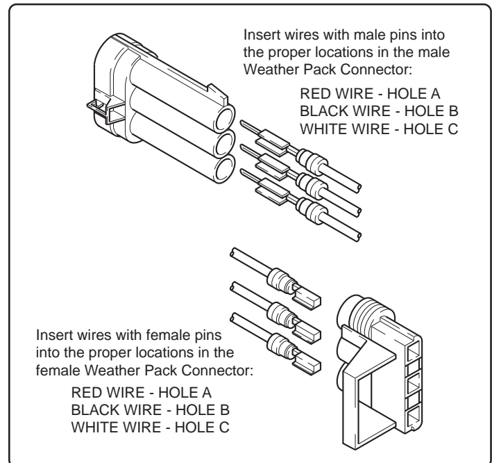
Figure B. Weather Pack Connectors for use with ETA225-WP
