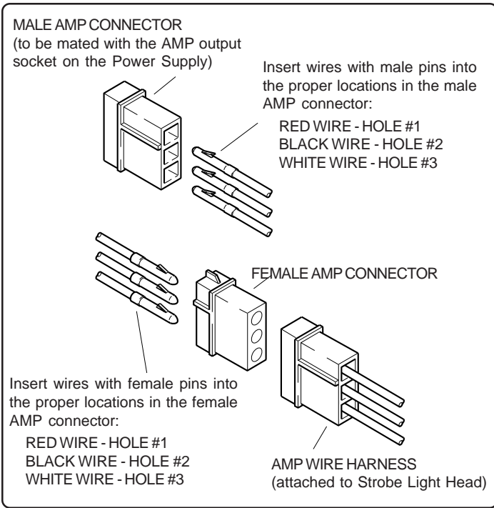
Figure C. Amp Connector for use with ETA225-P
