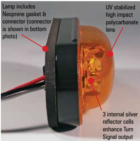
Three Gen3 LEDs brightly illuminate Turn Signal function to meet SAE certifications.
